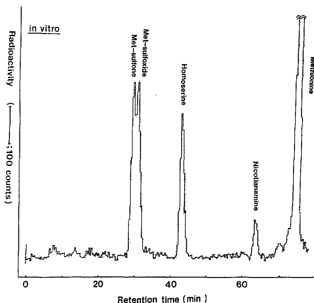
Fig. 3. Incorporation of L-methionine into nicotianamine by the crude protein fraction of N. megalosiphon in vitro. From the total volume of amino acid fraction recovered (600 \mu\text{l} ), 20 \mu\text{l} was injected into the HPLC at time 0 and detected with the on-line radioanalyzer at a time constant of 20 s
